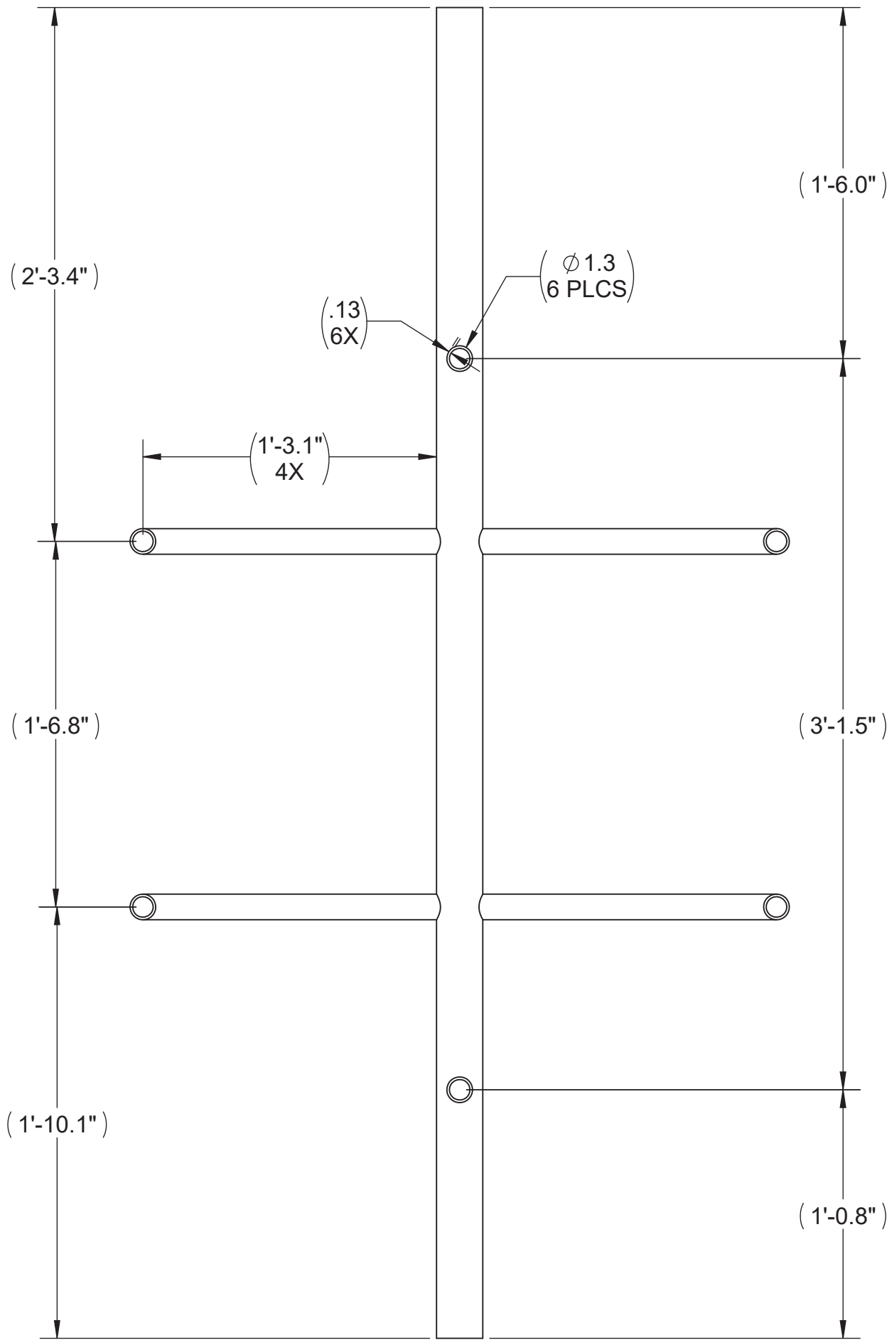
TOP VIEW
