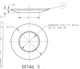
DETAIL S SCALE: 1/4" (SHOWN IN PLAN) (FROM SHEET 2)
