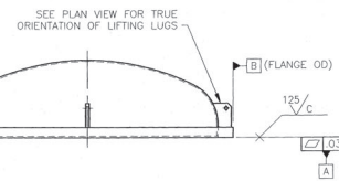
2 VESSEL HEAD WELDMENT SCALE: 3/4" = 1'-0"
