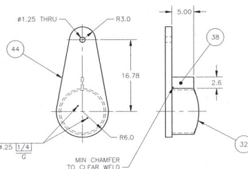
DETAIL V SCALE: 1/8" (2 REED) ROTATED 90° CW
