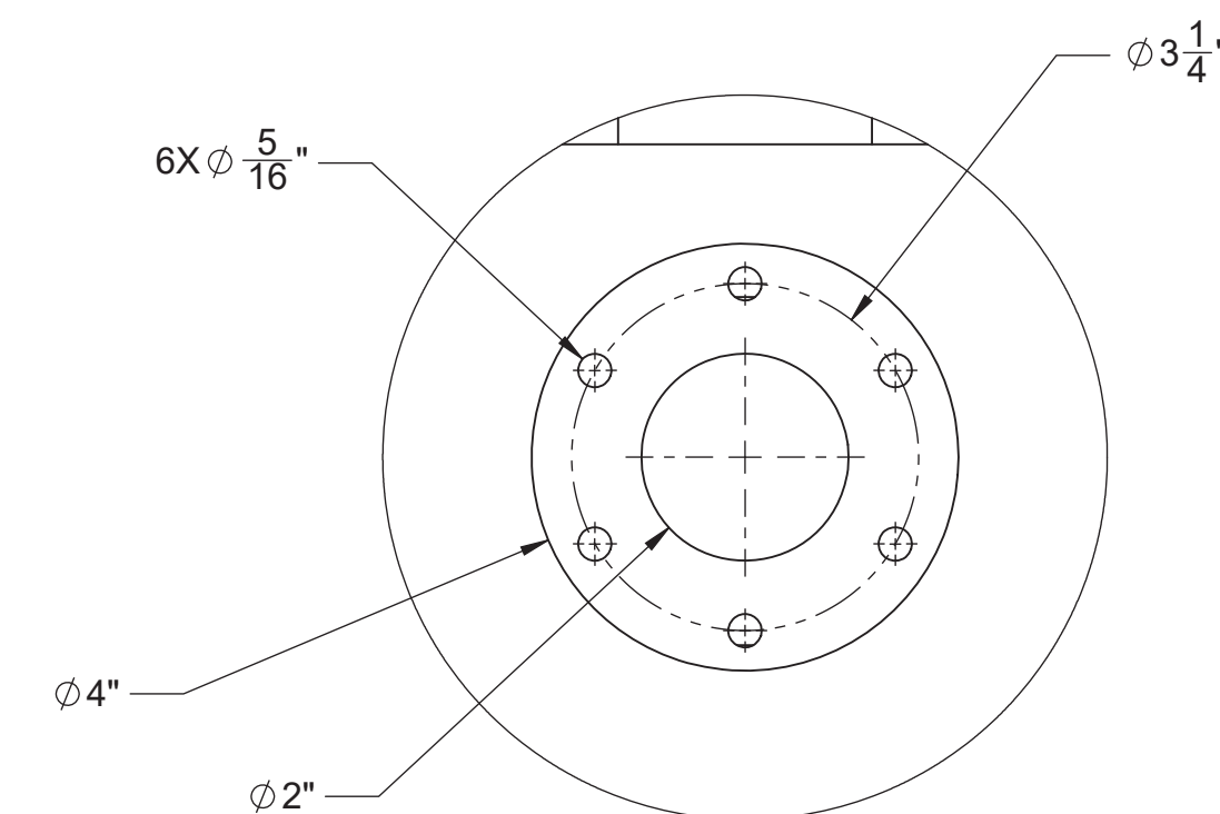
DETAIL I SCALE 1 : 2
