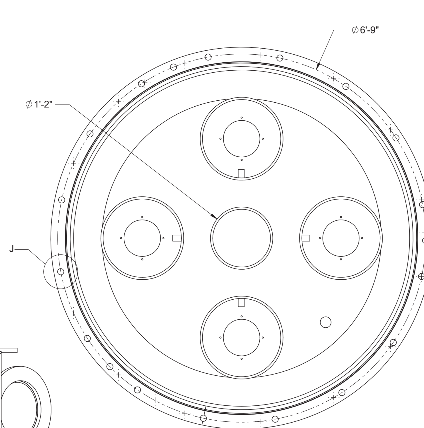
VIEW H-H
