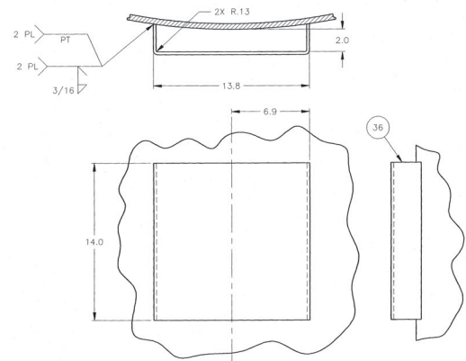
DETAIL H SCALE: 1/4 (FROM SHEET 2)
