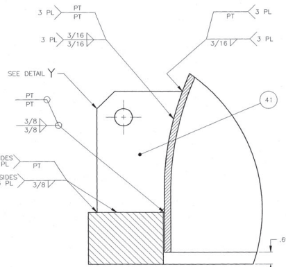
SECTION X-X SCALE: 1/2 (ROTATED 30° CCW)
