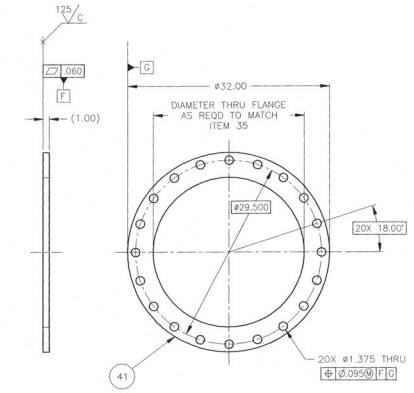
DETAIL U SCALE: 1/8 (FROM SHEET 2)
