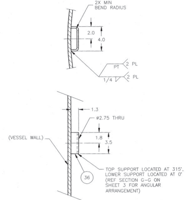
DETAIL Z SCALE: 1/4 (TYPICAL 2 PLACES)
