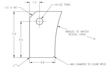
DETAIL Y SCALE: 1/2 (3 REQD)
