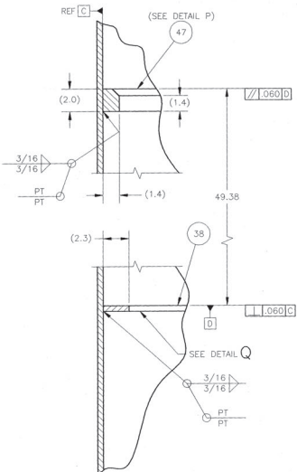
SECTION F-F SCALE: 1/4" (FROM SHEET 2)
