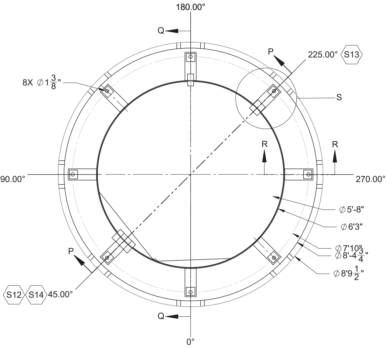
4 WESP LOWER SKIRT ASSEMBLY TOP VIEW
