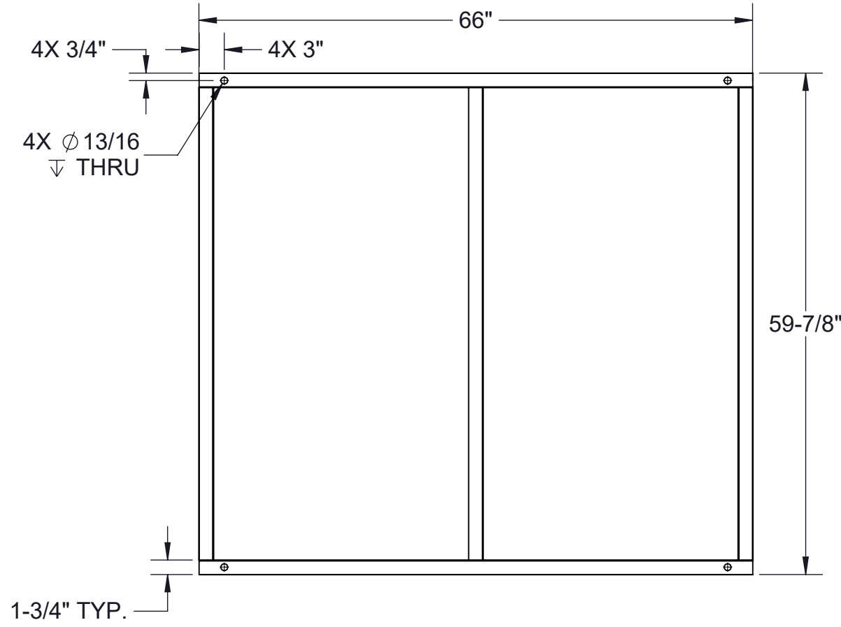
HEPA BASE BOTTOM VIEW SCALE: 1:16 GUSSET REINFORCEMENTS ARE 11 GA. T-304L SS SHEET
