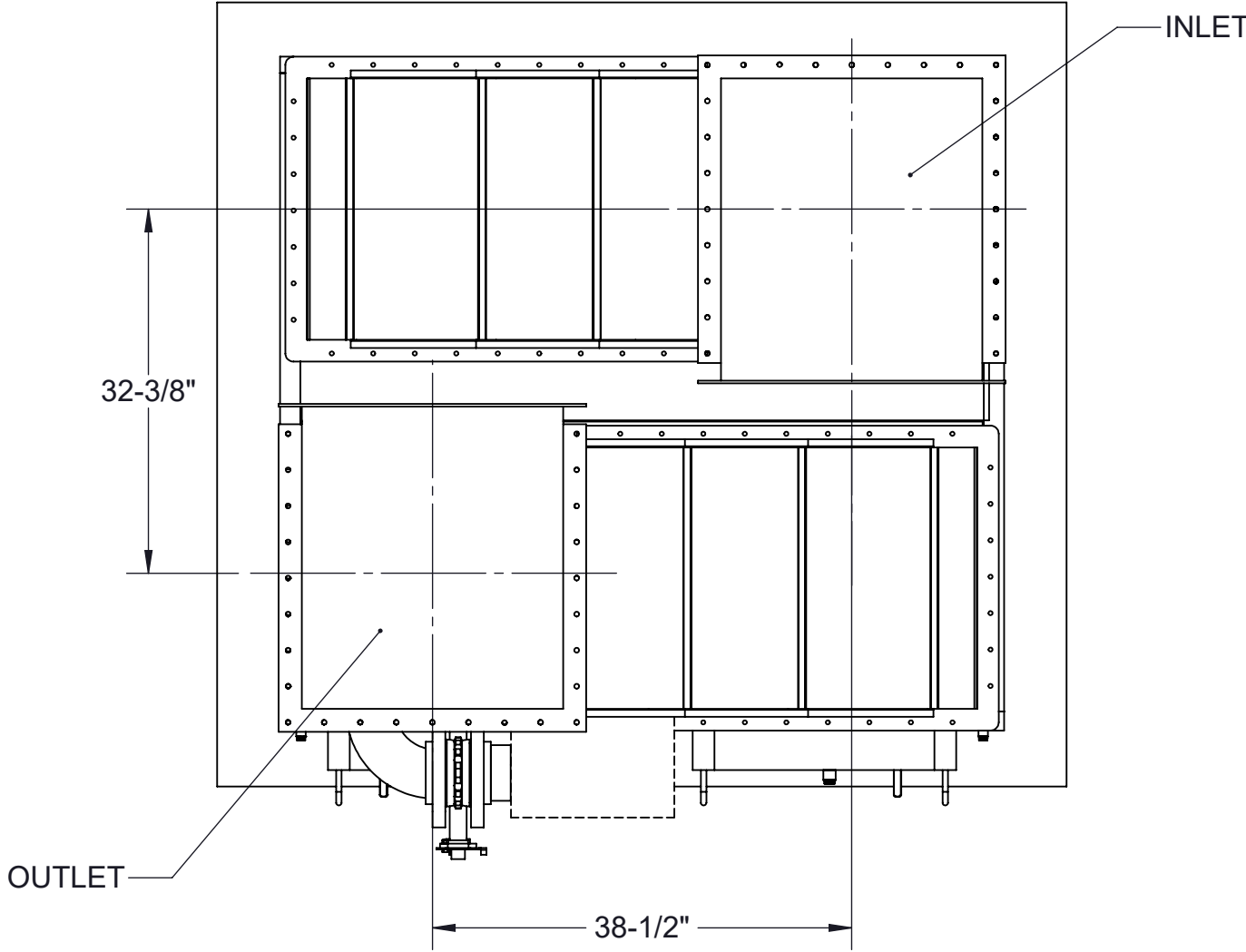
C5V HEPA INLET/OUTLET PLAN VIEW SCALE: 1:16
