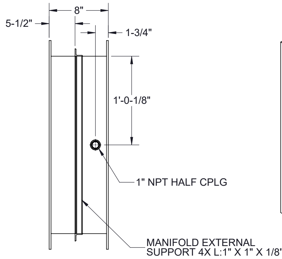
INLET TEST SECTION ASSEMBLY SCALE: 1:8 FOR INJECTION MANIFOLD PARTS AND WELDING SEE 24590-QL-POA-MKH0-00001-04-00048 & -00049
