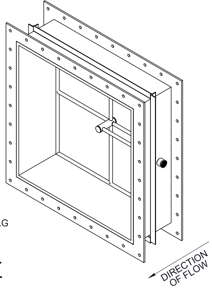
OUTLET TEST SECTION ASSEMBLY SCALE: 1:8 FOR INJECTION MANIFOLD PARTS AND WELDING SEE 24590-QL-POA-MKH0-00001-04-00046 & -00047
