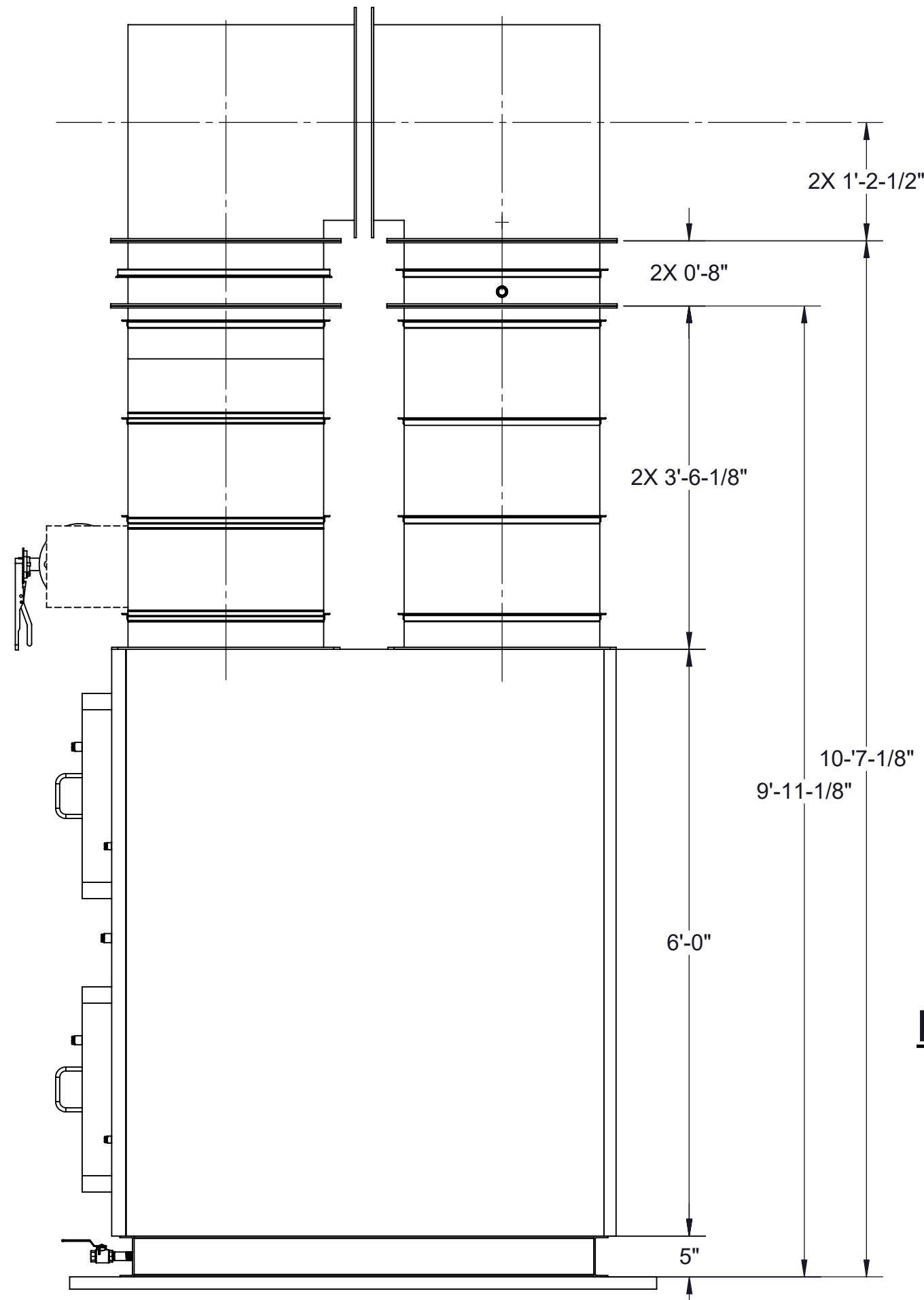
SECTION D-D SCALE: 1:16 ROTATED 180° VIEW LOOKING SOUTH INTAKE / EXHAUST DUCT, EXPANSION JOINTS AND DPR'S NOT SHOWN
