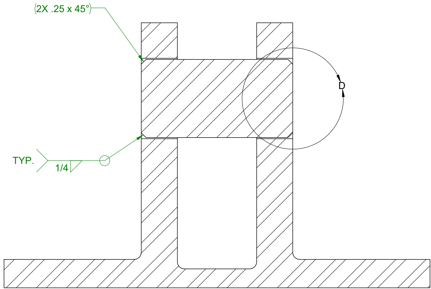
SECTION C-C
