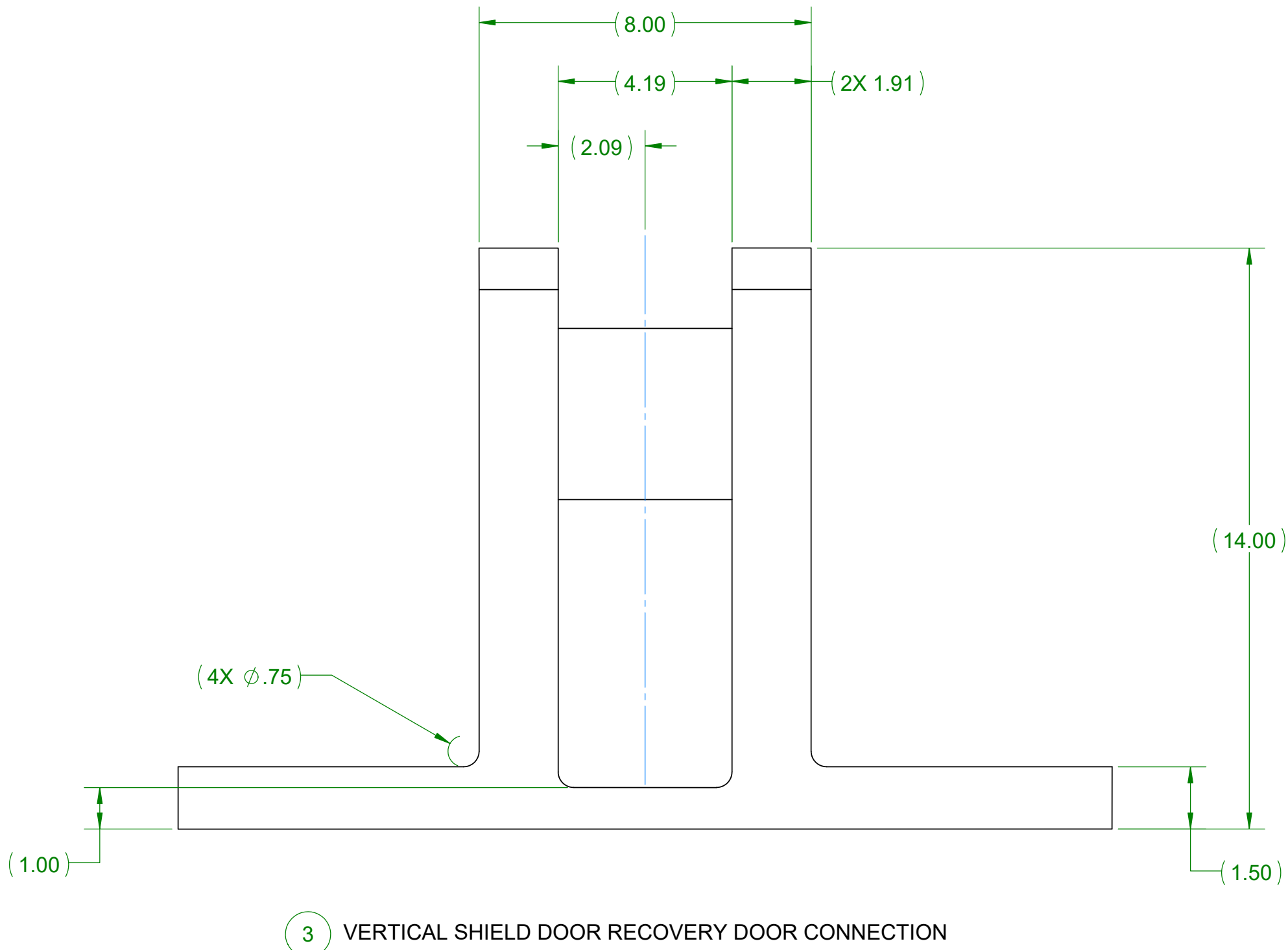
3 VERTICAL SHIELD DOOR RECOVERY DOOR CONNECTION
