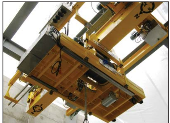
The bridge crane weighs 20,000 pounds, stands 9 feet tall and spans 10 feet in length and 16 feet in width. The crane will be used to handle spent HEPA filters from the Pretreatment Facility's filter cave.
